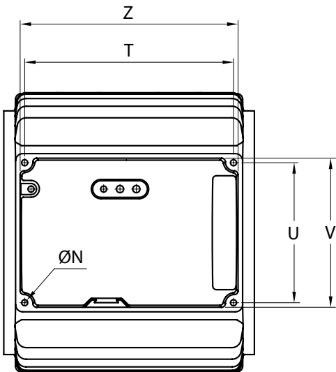
Header MEC 80 B3
