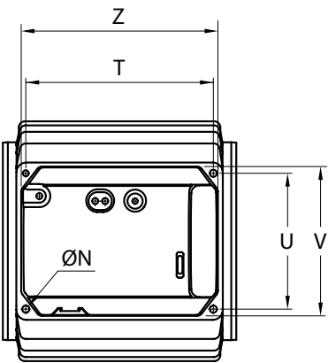
Header MEC 63 B3
