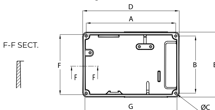
Long header MEC 71 B3-B5
