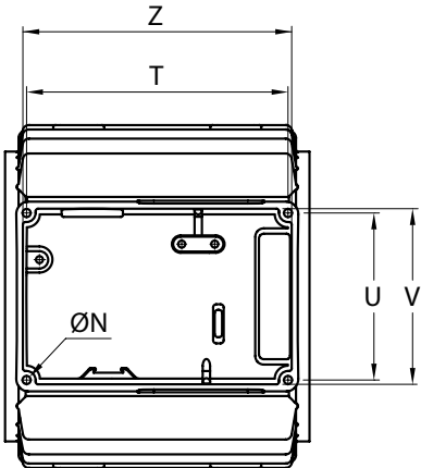
Header MEC 71 B3
