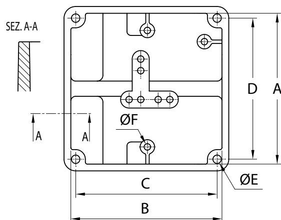
Basetta MEC 63-71-80 Basetta IEC 71-80-100
