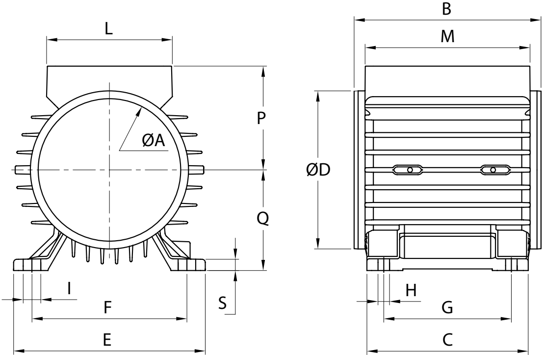
Basetta MEC 80 B3
