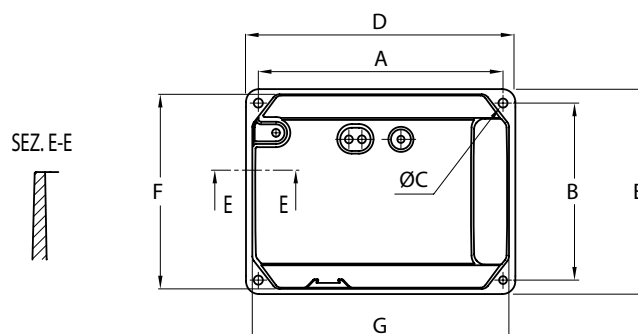
Basetta lunga MEC 63 B3-B5
