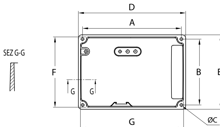
Basetta lunga MEC 80 B3-B5
