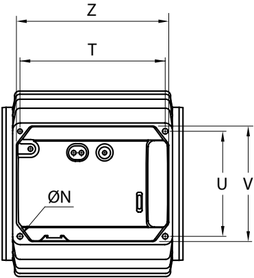
Basetta MEC 63 B3
