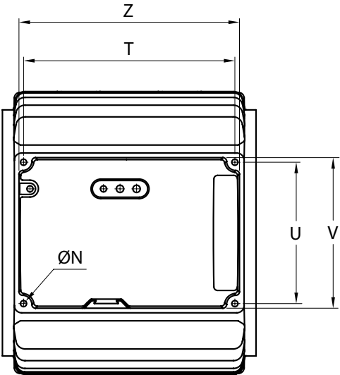
Basetta MEC 80 B3
