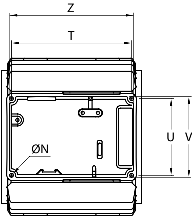
Basetta MEC 71 B3
